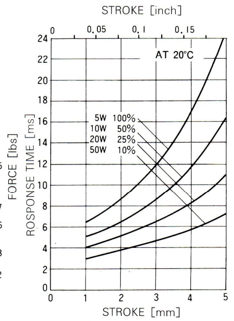
STROKE - RESPONSE TIME
