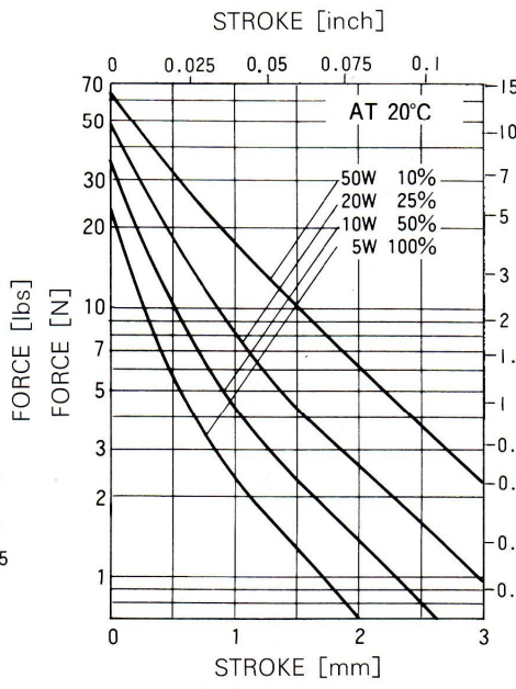
STROKE - FORCE (250F)
