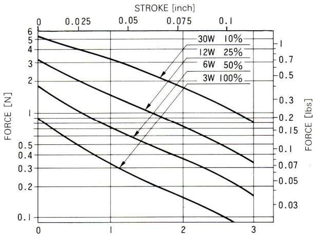
STROKE - FORCE
